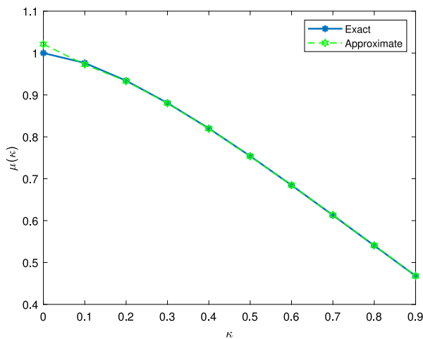
Fig. 3. Graph of exact and approximate solution.
