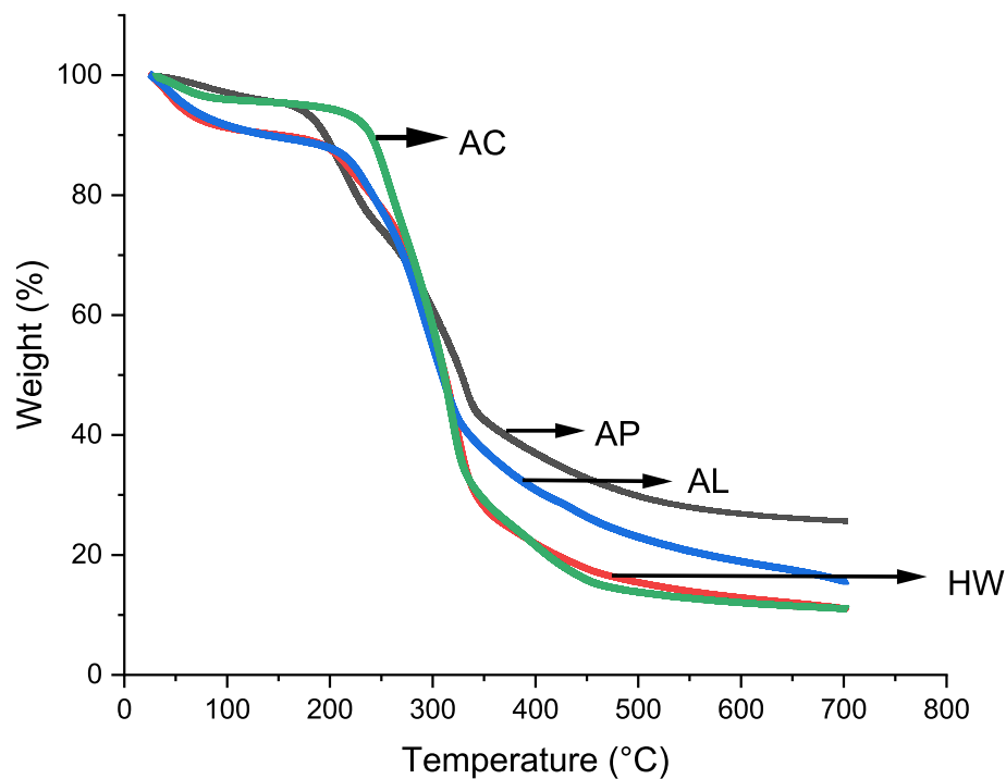
Fig. 3 Thermo gravimetric curves of apple pomace and extracted dietary fibre fraction
