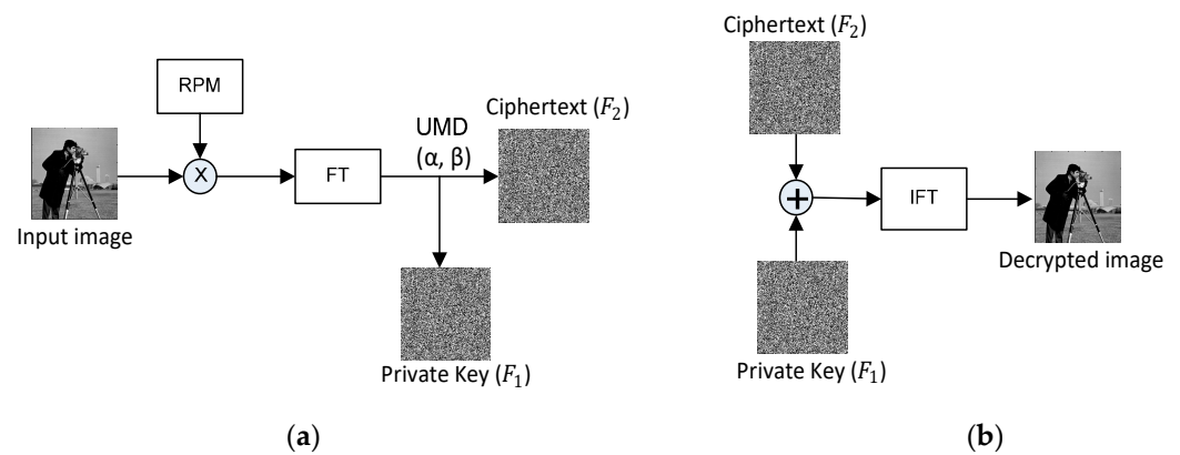
Figure 15. Basic flow chart of the (a) encryption and (b) decryption process of UMD.
