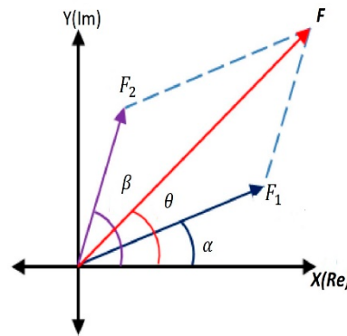
Figure 14. Geometrical representation of unequal modulus decomposition (UMD).
