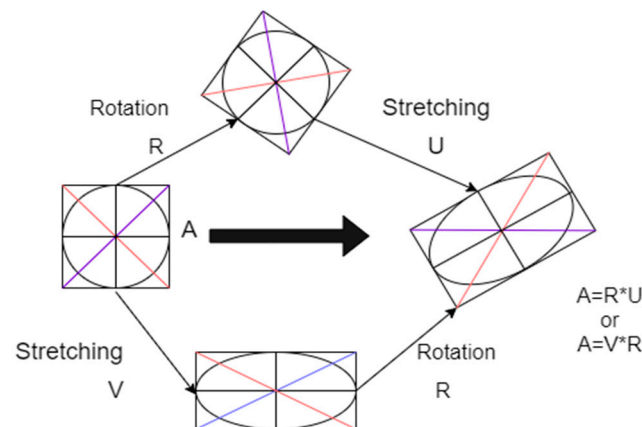
Figure 16. A geometrical illustration of polar decomposition.
