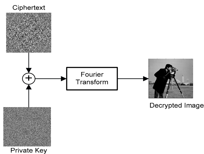
Figure 9. Schematic flowchart of the decryption process of a PTFT-based cryptosystem.
