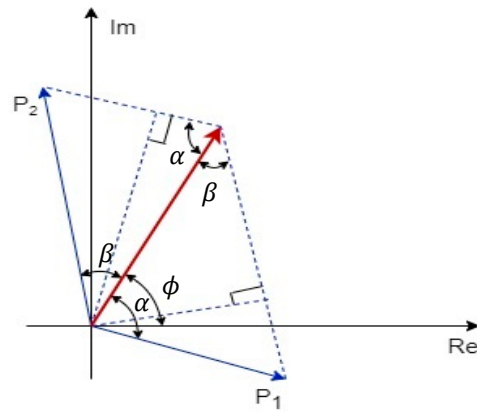
Figure 12. The geometrical representation of random modulus decomposition.
