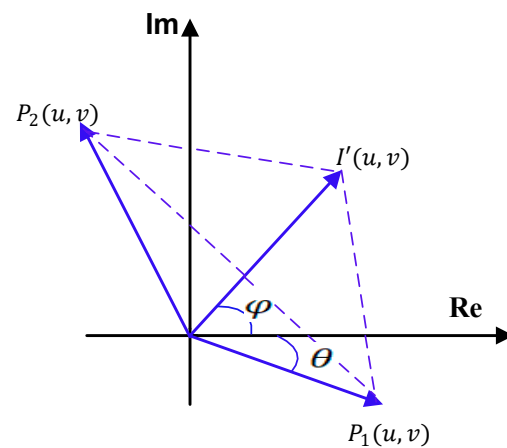
Figure 10. Graphical representation of the principle of equal modulus decomposition.
