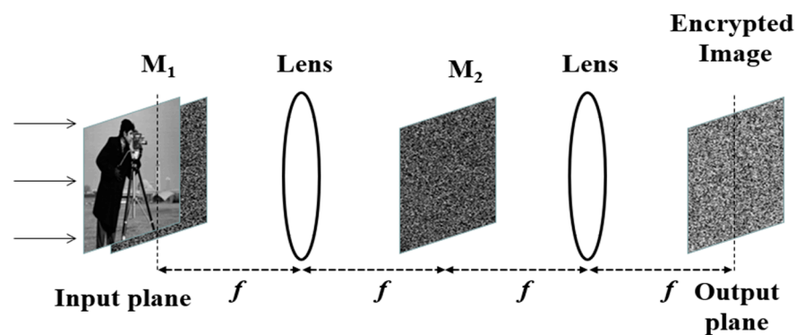
Figure 4. Optical image encryption process of DRPE proposed by Refregier and Javidi in 1995.
