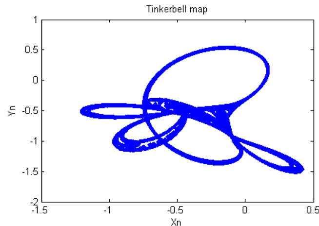
Figure 6. Attractor of the Tinkerbell chaotic map.
