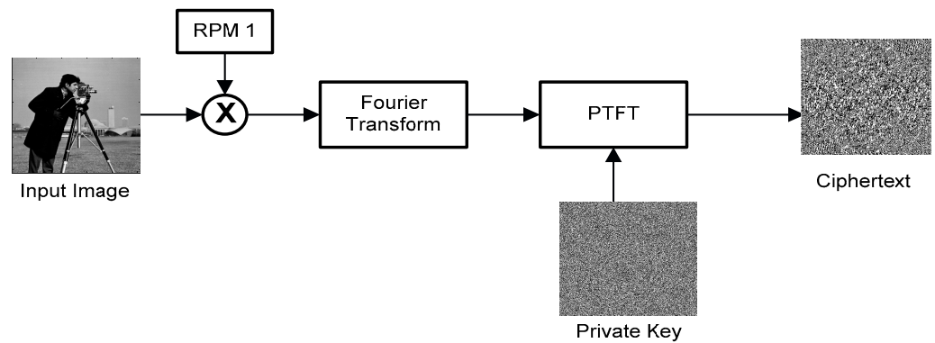
Figure 8. Schematic flowchart of the encryption process of a PTFT-based cryptosystem.
