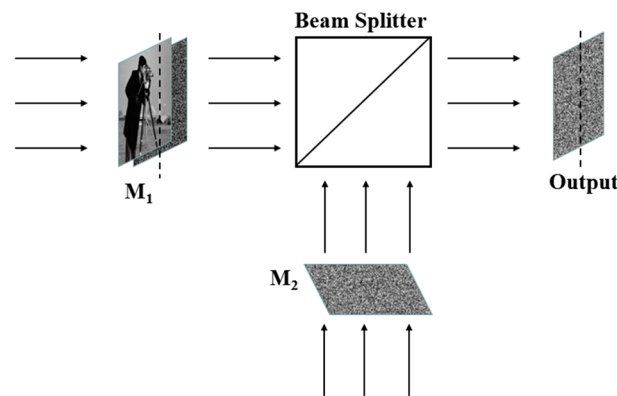
Figure 17. Optical image encryption using interference.
