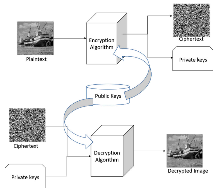
Figure 7. Schematic flowchart of an asymmetric cryptosystem.
