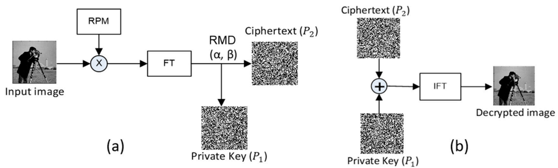
Figure 13. Basic flow chart of the (a) encryption and (b) decryption process of EMD.
