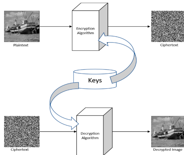
Figure 5. Diagrammatic flowchart of symmetric key cryptosystems.
