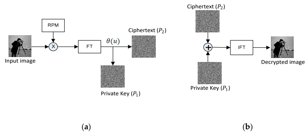
Figure 11. Basic flow chart of the (a) encryption and (b) decryption process of EMD.
