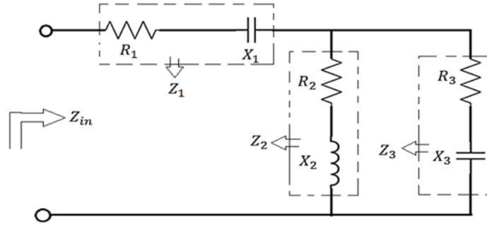
Figure 3. Electrical equivalent impedance circuit of quantum antenna for phasor representation.
