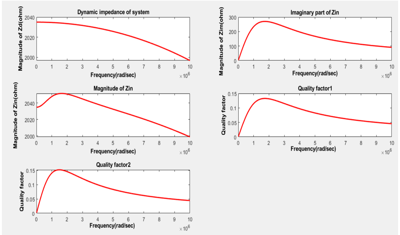
Figure 10. Simulated graph of all parameters of QA at L_2 = 1210\text{e} - 6\text{H} , C_1 = 25\text{e} - 15\text{F} , C_3 = 143\text{e} - 15\text{F} with R_1 = 1000\ \Omega , R_2 = 1035\ \Omega , and R_3 = 1065\ \Omega .
