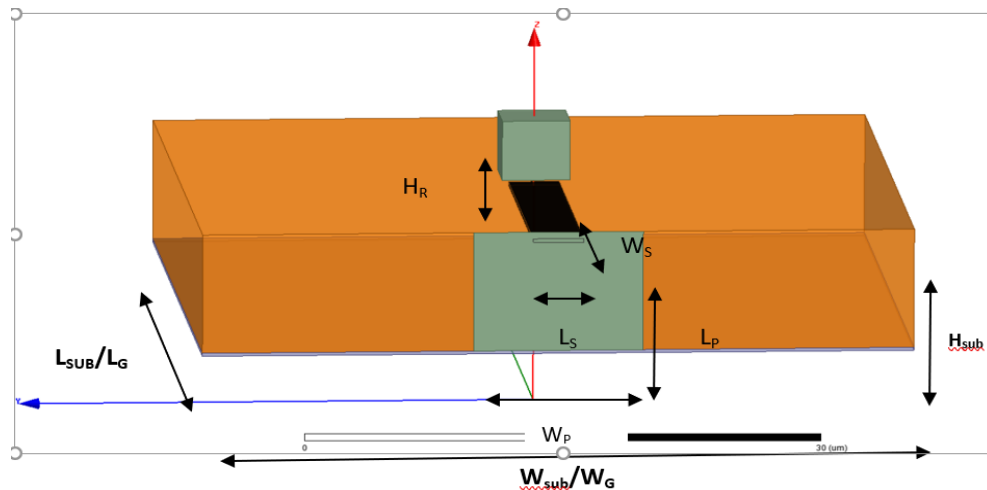
Figure 14. Quantum rectangular DRA.
