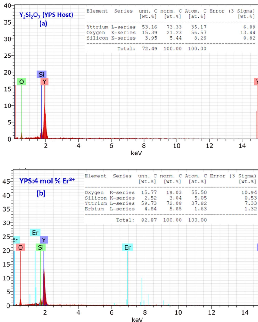
Fig. 6 EDX profiles of (a) the \text{Y}_2\text{Si}_2\text{O}_7 and (b) \text{Y}_{1.96}\text{Si}_2\text{O}_7:4 \text{ mol \% } \text{Er}^{3+} phosphor. The inset represents the chemical composition of the respective samples.
