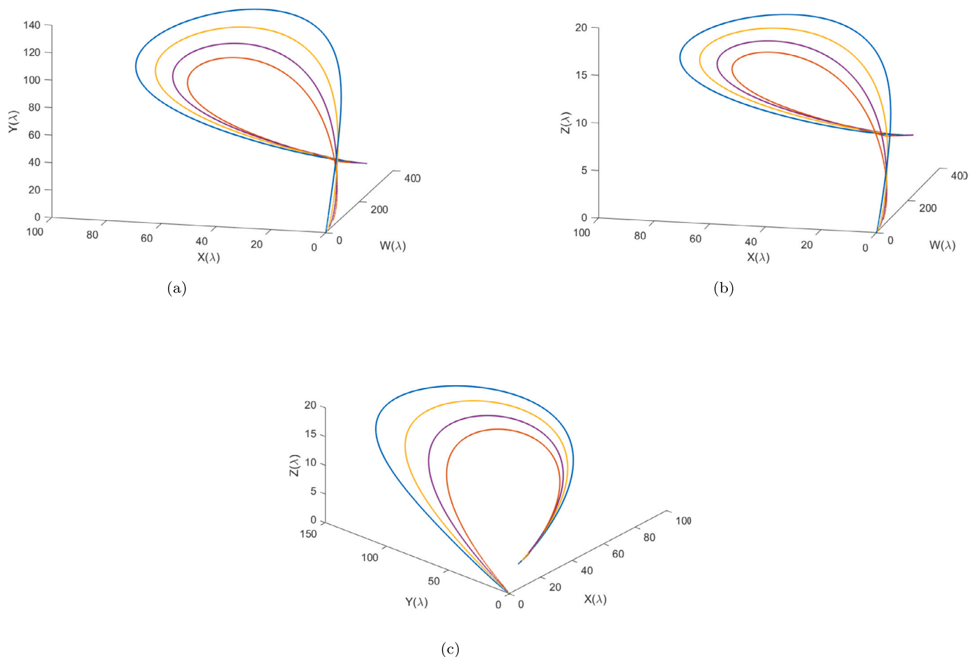
Fig. 5. The presence of attractors, specifically with the given parameters \gamma=0.04 , \eta=0.009 , \rho=0.13869 , \chi=0.06654 , \mu=0.09281 , \varepsilon=0.88187 , indicates the enduring coexistence and stability of the entire population over time.
