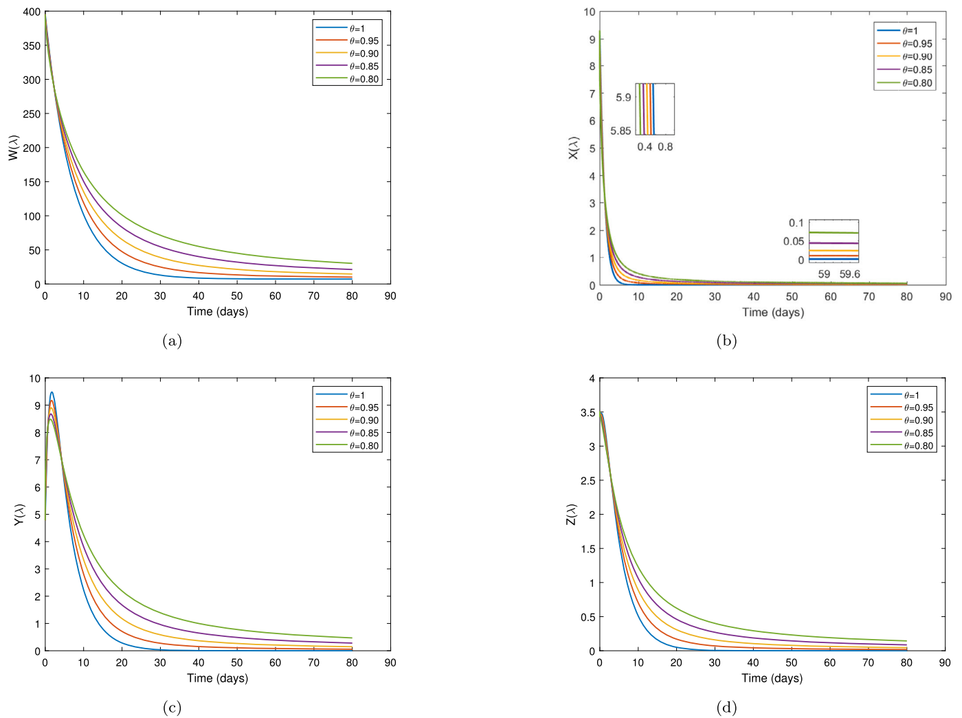
Fig. 2. Simulation of W(\lambda) , X(\lambda) , Y(\lambda) , Z(\lambda) with \gamma = 1 , \eta = 0.0009 for different fractional order of \theta .
