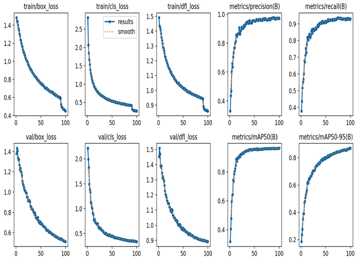
Fig. 8. Results of the proposed model indicate the performance and stability. All the training and validation loss functions decrease as the epochs increase. The mAP50 metric crossed 0.9 in the first 20 epochs, increased constantly, and finally reached 0.965.
