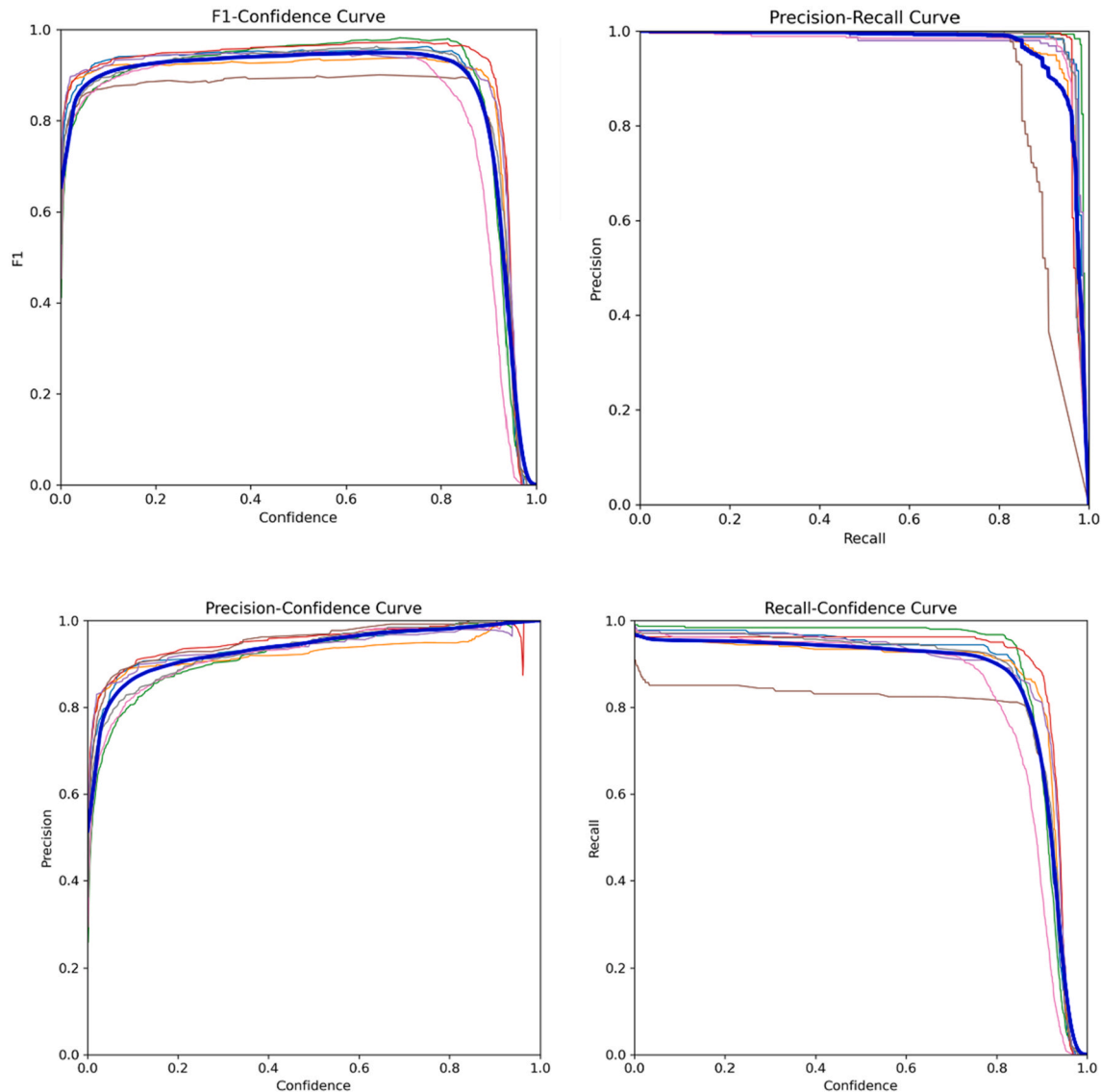
Fig. 10. The training graphs display the F1 confidence curve, precision-recall curve, precision confidence curve, and recall confidence curve.
