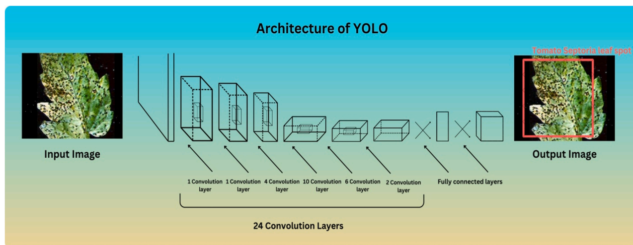
Fig. 3. Architecture of Yolo model that integrates state-of-the-art techniques in deep learning and computer vision, including advanced feature extraction layers, fully connected layers optimized anchor box clustering, and improved training strategies.
