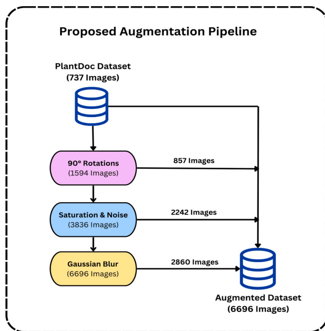
Fig. 7. Schematic augmentation pipeline.
