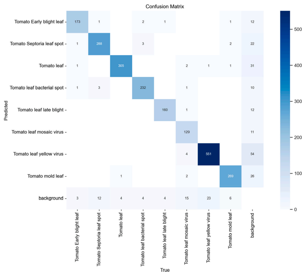
Fig. 9. Confusion matrix. The principle diagonal represents all the true predictions and contains most of the values. A small number of false positives and false negatives do not require much attention.
