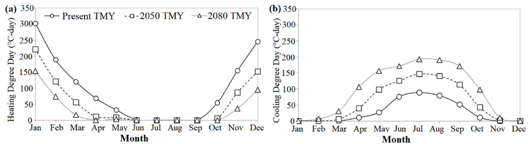
Fig. 6. (a) Monthly heating degree day (HDD) and (b) cooling degree day (CDD) for the different climatic scenarios (base temperature 18^{\circ}\text{C} ).
