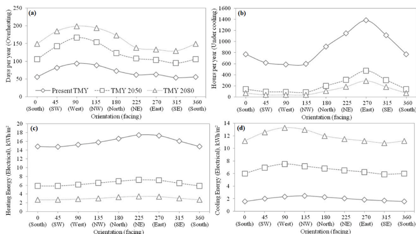
Fig. 15. Variation of (a) CIBSE overheating (days per year); (b) Indoor under cooling hours (hours per year); (c) heating energy demand; and (d) cooling energy demand with different orientation of the building under different climatic scenarios.
